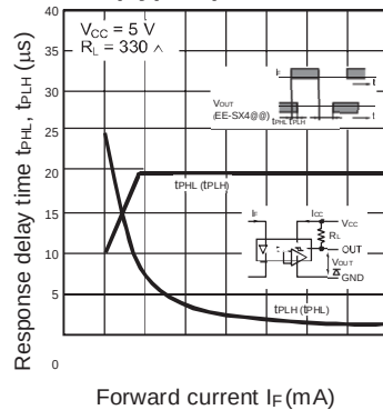
Response Delay Time vs. Forward Current (Typical)
