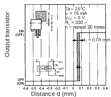
Repeat Sensing Position Characteristics (Typical)
